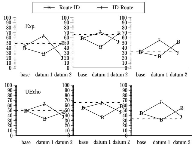
Figure 4: Belief evaluation results. The dashed lines indicate the Bayesian values of base rate and final belief.
